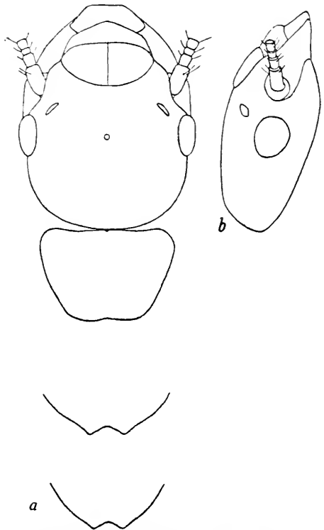
FIGURE 7.— Microcrotermes becconi , new species: a, Dorsal view of head, pronotum, mesonotum, and metanotum; b, lateral view of head. Winged adult. \times 40
